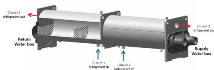
Figure 2 – CHIL Evaporator
